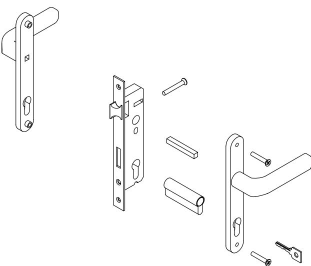
Mortise Lock
