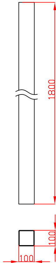
100X100-1800MM Inground Post
