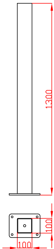
100X100-1300MM Flanged Post
