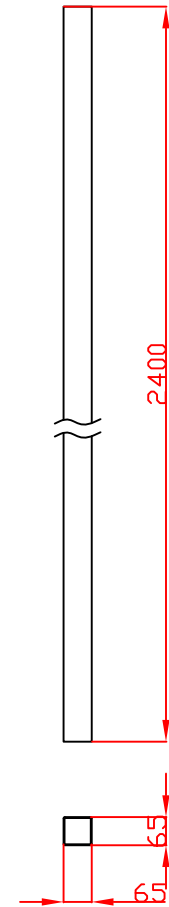
65x65-2400mm Inground Post
