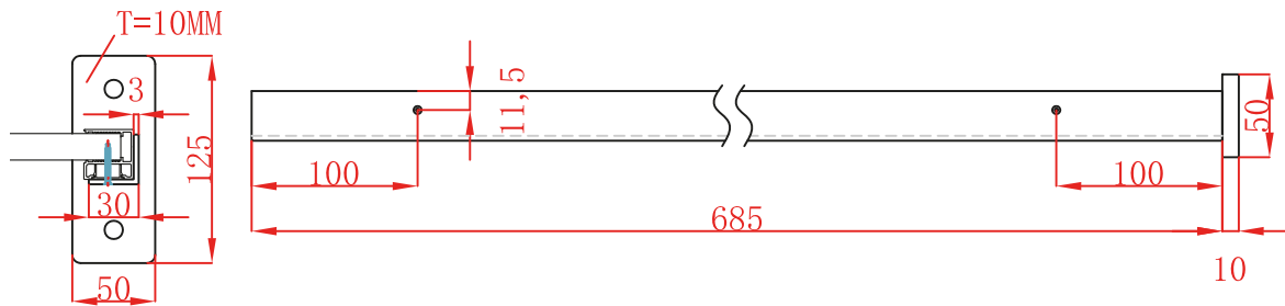
Angle Base Bracketx2pcs
